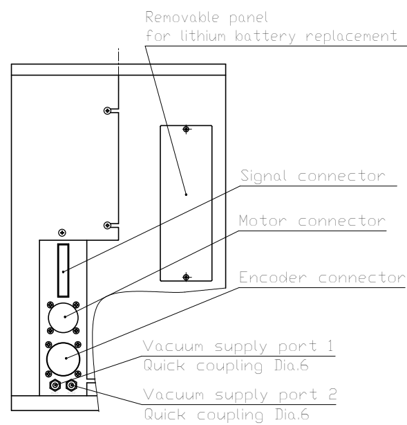
Details of connection
